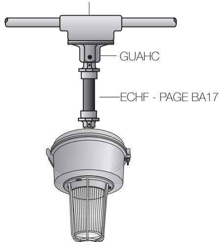
TYPE GUA OUTLET BOX - PAGE BA18
