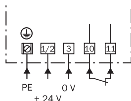
Figure 14: Assignment of the sensor contacts, transmitter
