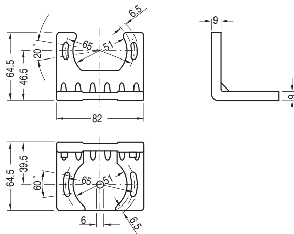
Figure 24: Mounting bracket (440L-AMBRK4)
