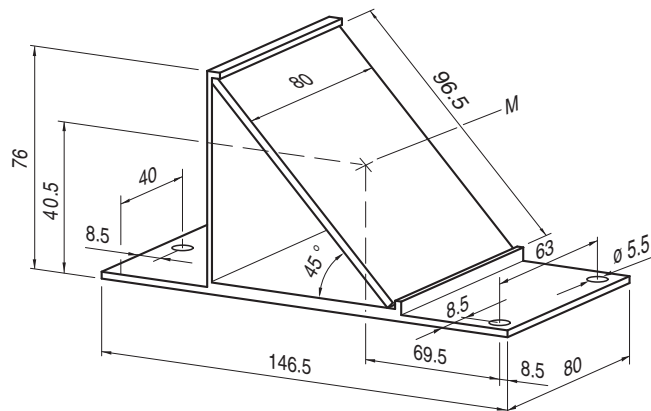
Figure 23: Corner mirror (M = Middle of the mirror surface) (440L-AMIRR2)
