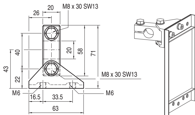
Figure 21: Bracket for corner mirror 1 (440L-AMBRK1)
