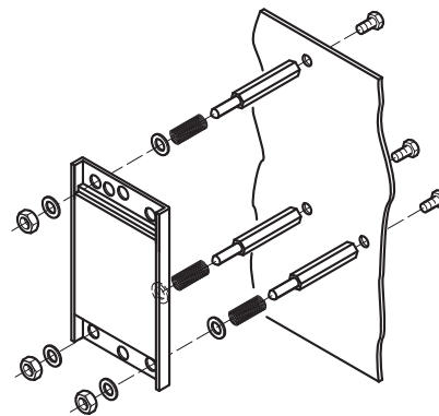
Figure 22: Spring fastening for corner mirror (440L-AMKIT)
