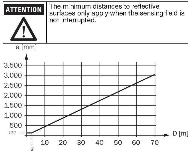
Figure 7: Graph, minimum distance from reflective surfaces
