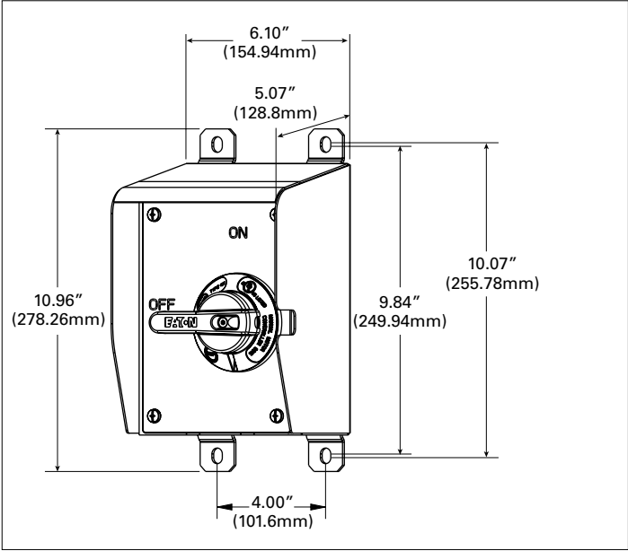
Figure 1. AHDS30SSR Dimensions
