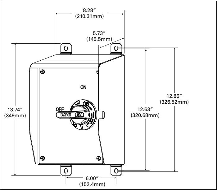
Figure 2. AHDS60SSR and AHDS100SSR Dimensions
