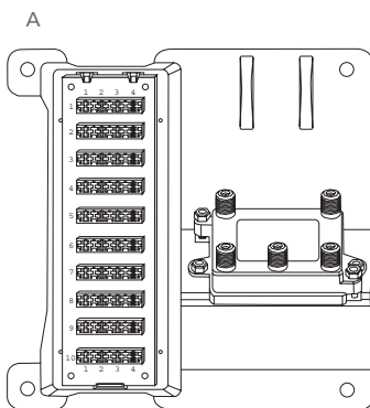
[ A ] Telephone & 4-way Video 47603-1G4
