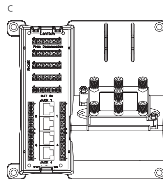
[ C ] 4 Telephone, 4 Data & 6-way Video 47603-DP6
