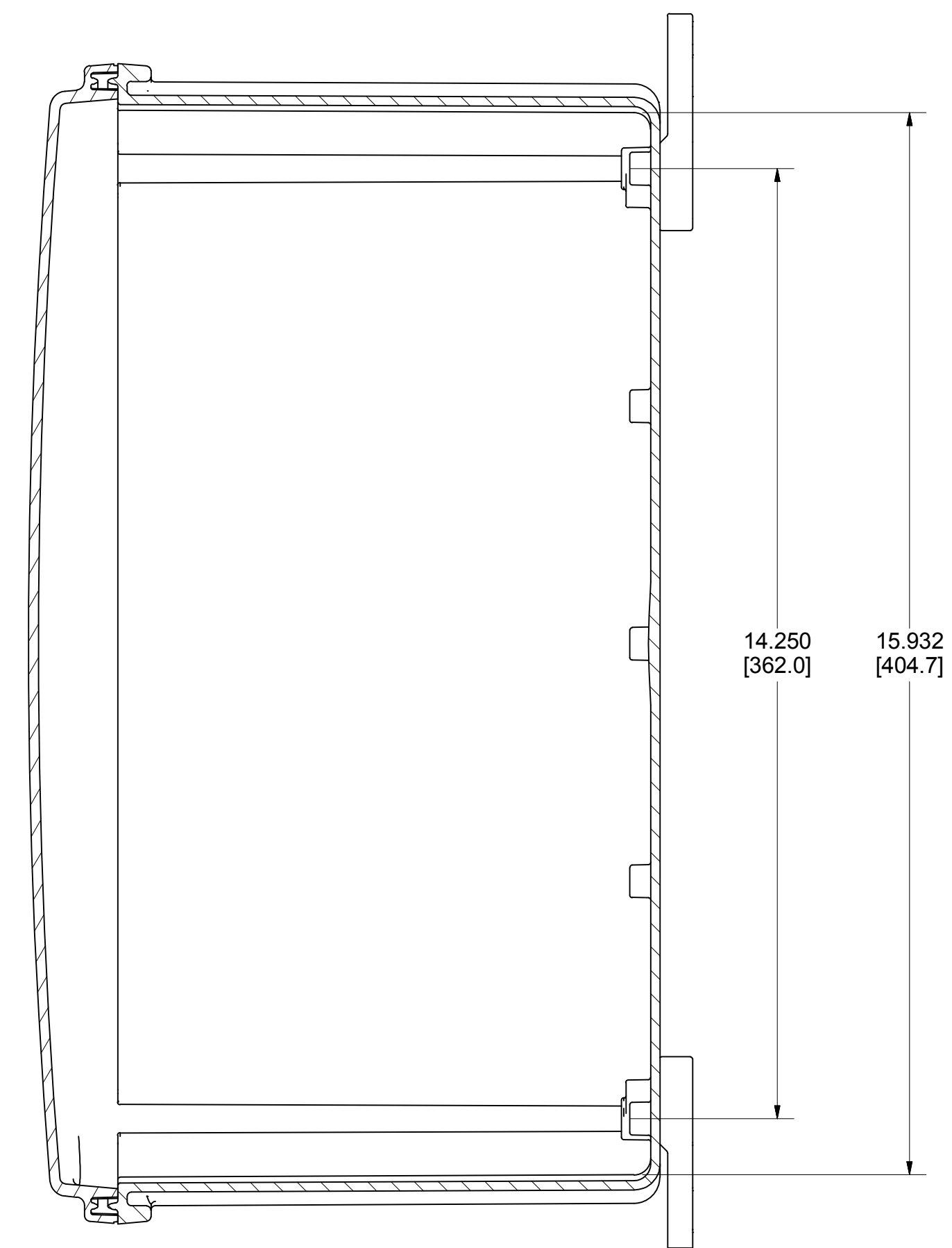
SECTION B-B
