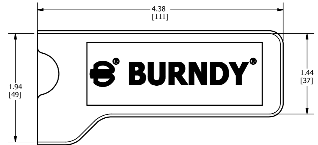
WIRE MIKE COVER
