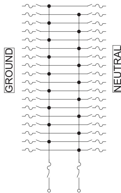
Single-phase, 3 wire fused main disconnect
