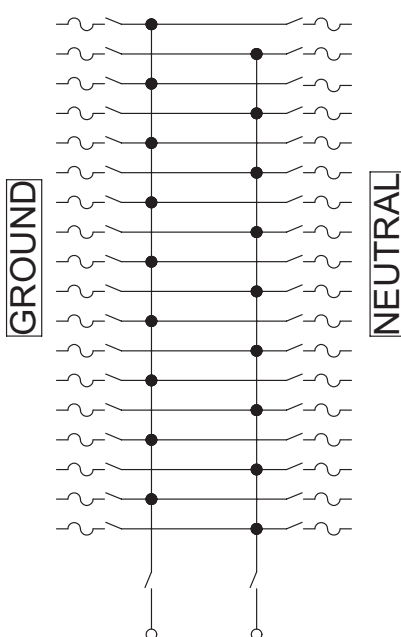
Single-phase, 3 wire non-fused main disconnect
