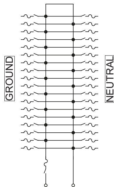
Single-phase, 2 wire fused disconnect
