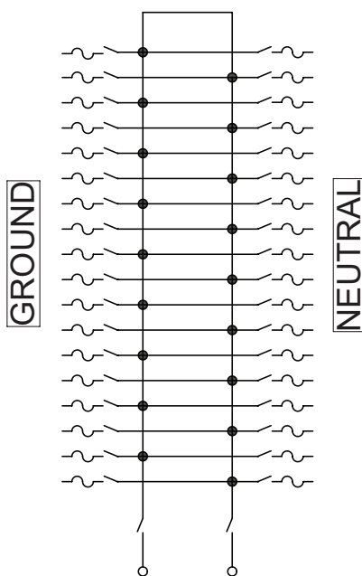
Single-phase, 2 wire non-fused disconnect
