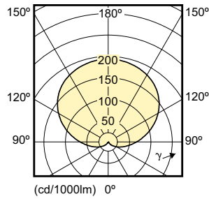
10.5-75W, 13-75W /830 3000K 220-240V
