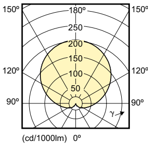
Bulb G25 120V 500lm 150D WW E26 ND
