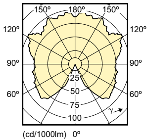
ND 6.5-40 W A60 CL WW 2700 K
