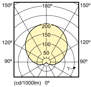
9-60 W /830 3000K 220-240V
