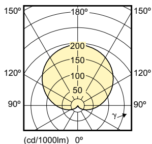
4-32 W, 5-32 W /830 3000K 220-240V
