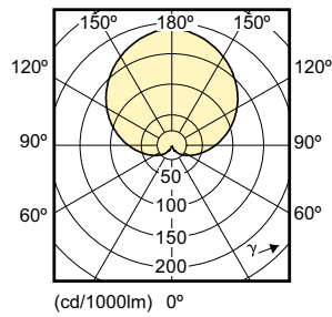
40W, 60W A60
