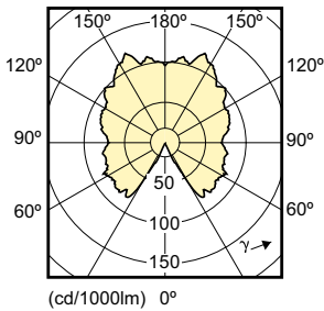
ND 9.5-60 W A60 CL WW 2700 K
