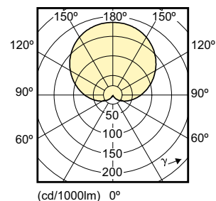
6.5-48 W /830 3000K 220-240V
