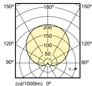
9-60W E27 /827 2700K 220-240V
