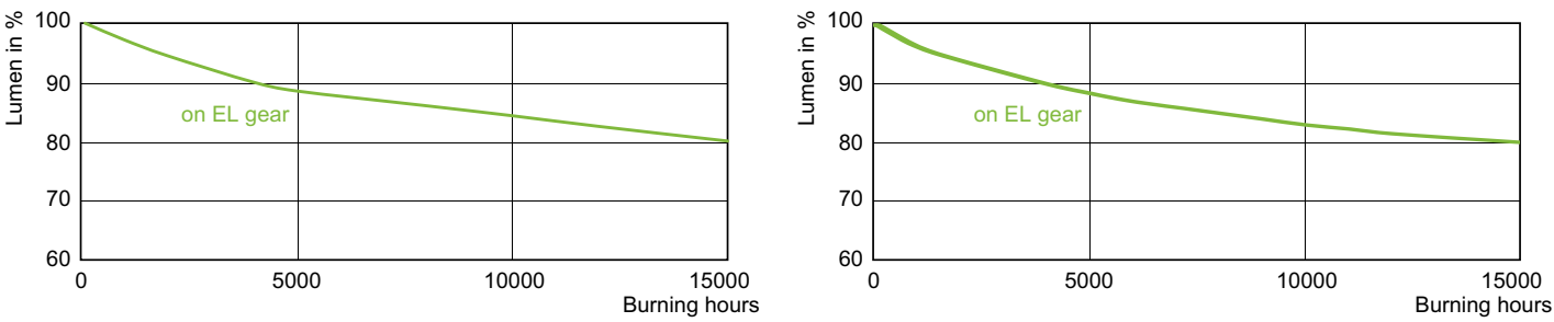
CDM-T Elite 50W & 70W Lumen Maintenance /930
