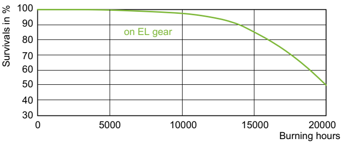
CDM-T Elite 35W, 50W, 70W, 100W Life Expectancy /930
