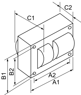
MH BAL 400W M59 480V/120T KIT
