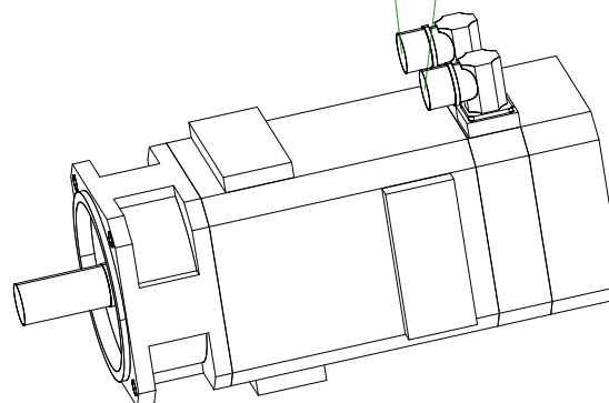
17-pole plug for optical encoder 6-pole plug size 1 for power and brake
