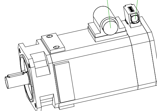
6-pole plug size 1.5 for power and brake
