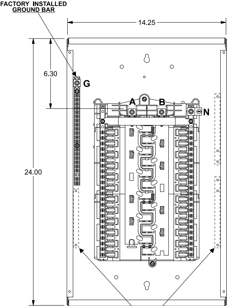
VIEW SHOWN WITH TRIM ASSEMBLY REMOVED
