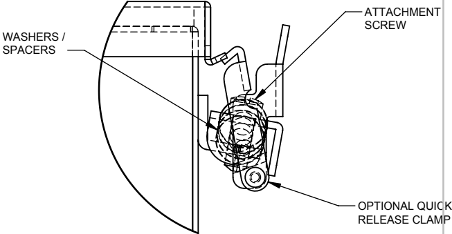
OPTIONAL CLAMP DETAIL (SUFFIX "-QR")
