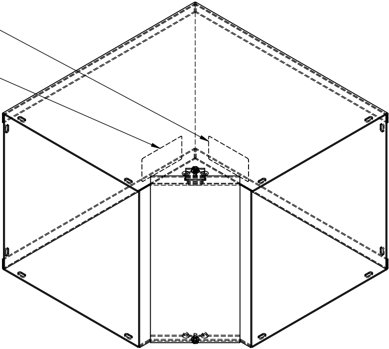
ISOMETRIC VIEW
