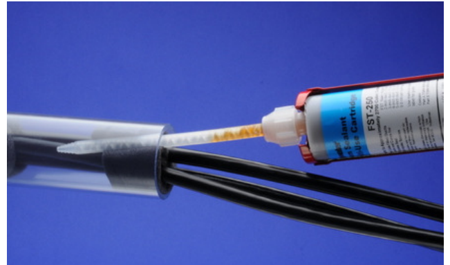
The FST™ Sealant comes in a caulking style (one plunger) tube. Package allows multiple seals. Mixing is done in the nozzle as the sealant is injected.
