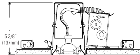
2025WH/2000LVNT Low Voltage Remote Transformer
