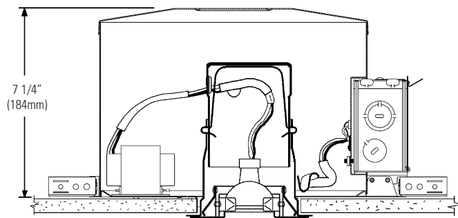
2025WH/2004ICV/N Lytefining™ AirSeal® Insulated Ceiling
