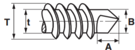
5/16 & 3/8 Diameter #3 Point
