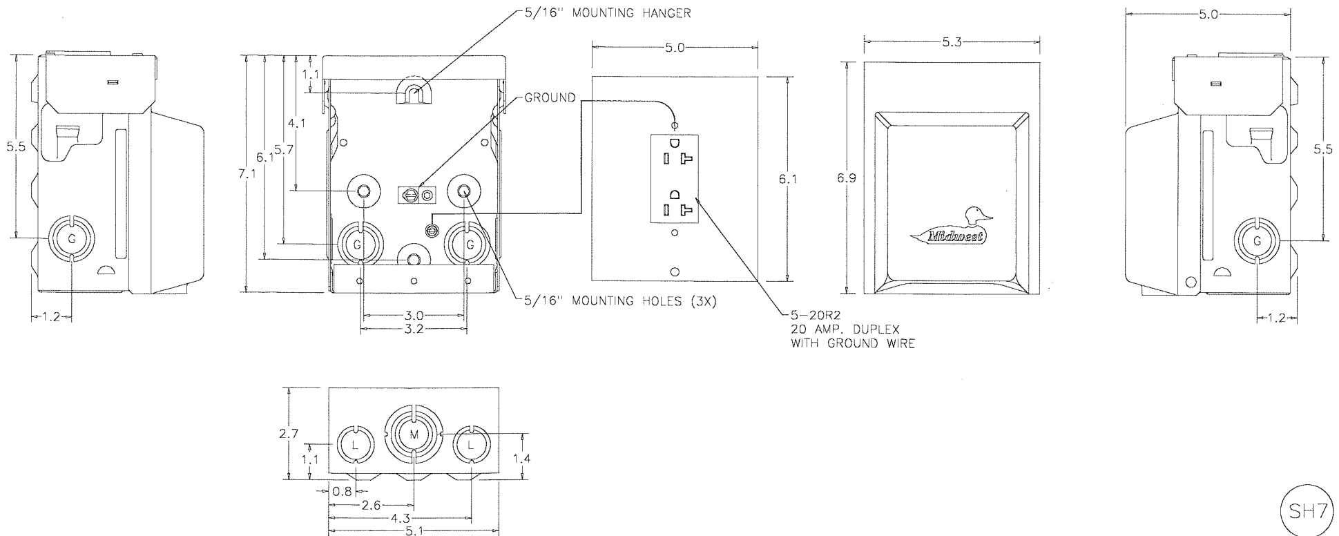
KNOCKOUT TABLE:
