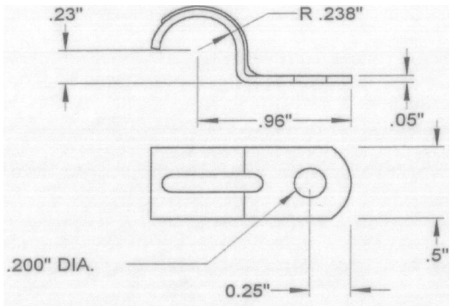
One Hole Strap 3/8" (Peco Part Numbers P38BX and P38BXJ)
