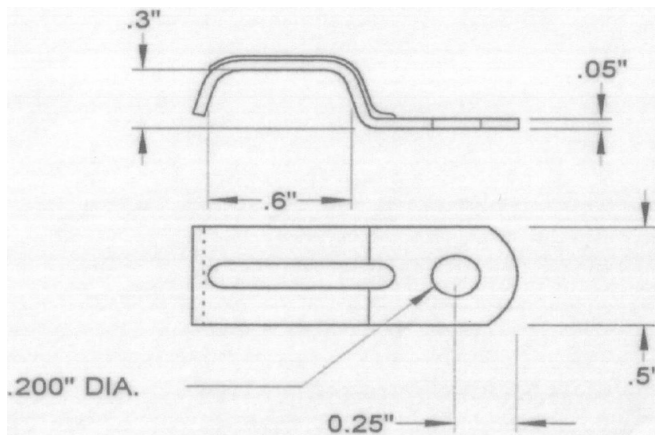
One Hole Romex Strap (Peco Part Number P713J)
