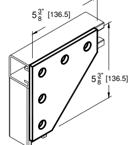
5 Hole Corner Gusset Plate
