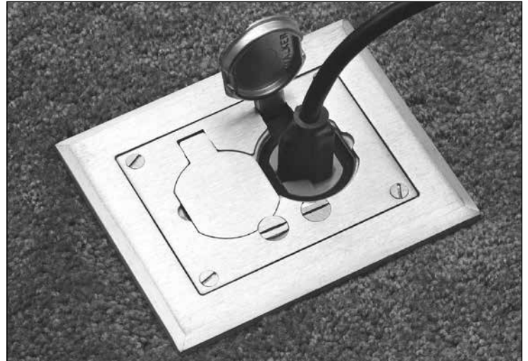
Source 1 Single-Gang Flush Service Fittings in brass.
