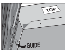
Figure 1 Face of wall can must extend ½ inch or ⅝ inch from face of stud to allow for thickness of sheetrock.
