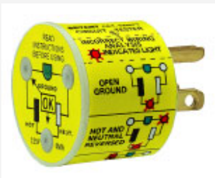
Straight Blade Receptacle Polarity Tester.
