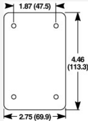
FS Type Box Blank Cover.
